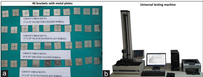
Figure 3: Metal plates with testing apparatus, (a) central incisor brackets mounted on metal plates and (b) universal testing machine is used for checking frictional resistance
